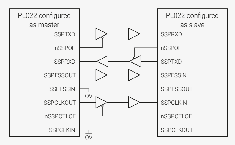
Figure 97. PrimeCell SSP master coupled to a PL022 slave
