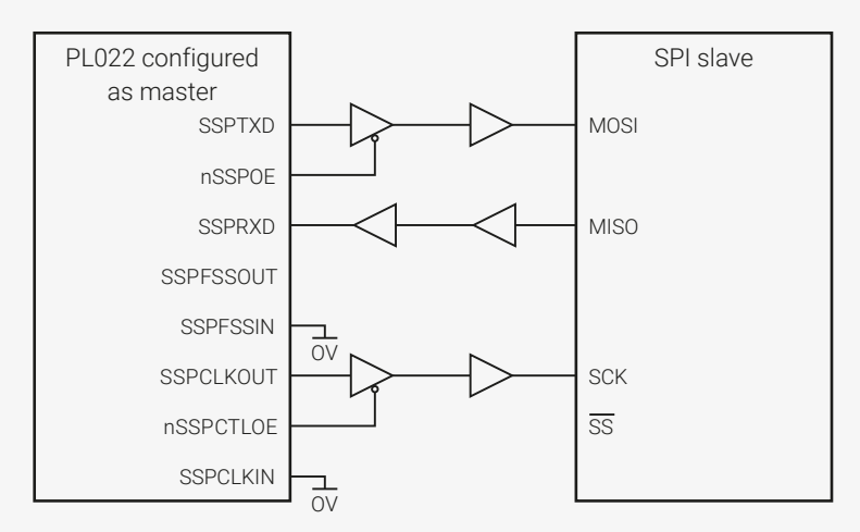
Figure 98. PrimeCell SSP master coupled to an SPI slave
