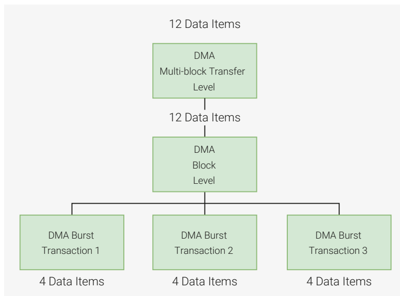
Figure 160. Breakdown of DMA Transfer into Burst Transactions. Block size, DMA\_CTLx.BLOCKS\_TS = 12 . Number of data items per source burst transaction, DMA\_CTLx.SRC\_MSIZE = 4 . SSI receive FIFO watermark level, SSI.DMARDLR + 1 = DMA\_CTLx.SRC\_MSIZE = 4
