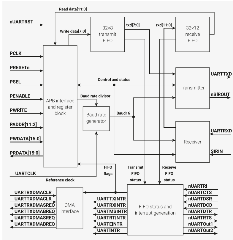
Figure 57. UART block diagram. Test logic is not shown for clarity.
