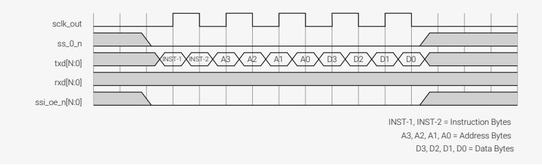
Figure 155 describes a DDR write transfer where instruction, address and data all are transferred in DDR format.
