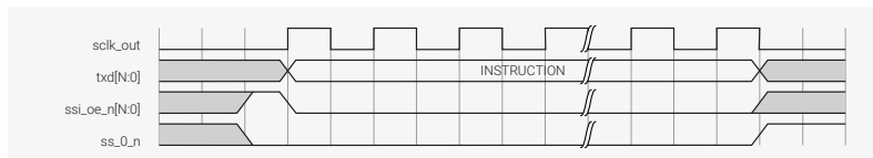
Figure 147. Instruction only transfer in enhanced SPI Format
