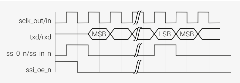
Figure 129. SSP Serial Format Continuous Transfer
