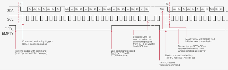
Figure 78. Master Receiver – First Command Loaded After Tx FIFO Allowed to Empty/Restart Bit Set
