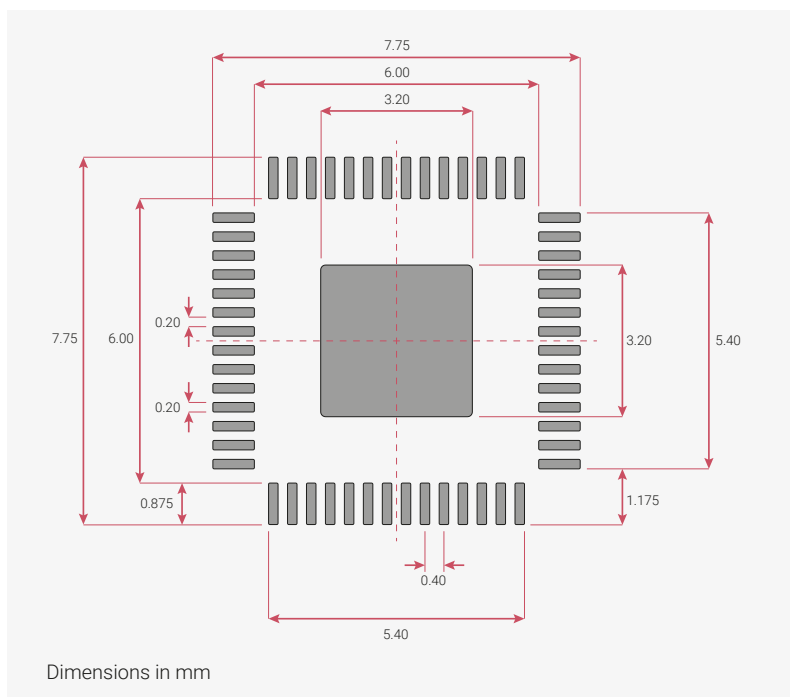
Figure 163. Recommended PCB Footprint for the RP2040 QFN-56 package
