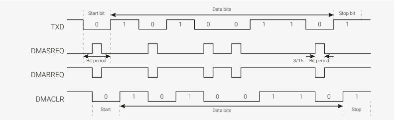
Figure 59. UART character frame.
