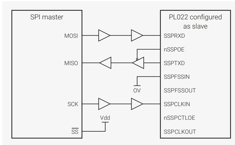
Figure 99. SPI master coupled to a PrimeCell SSP slave
