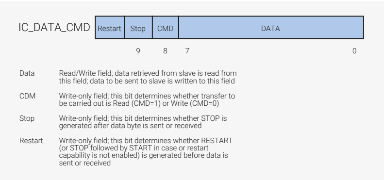
Figure 70. IC_DATA_CMD Register
