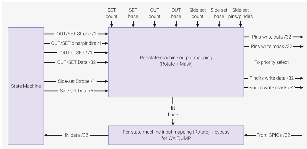
Figure 46. The state machine has two independent output channels, one shared by OUT/SET, and another used by side-set (which can happen at any time). Three independent mappings (first GPIO, number of GPIOs OUT, SET and side-set are directed to. Input data is rotated according to which GPIO is mapped to the LSB of the IN data.
