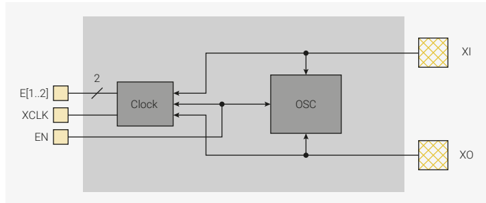
Figure 31. XOSC overview
