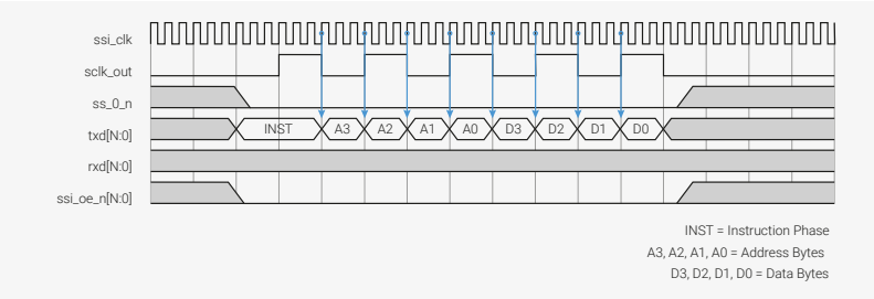
Figure 156 shows the default behavior in which the transmit and driving edge of the data is the same.
