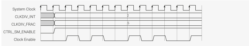
Figure 45. Fractional clock division with an average divisor of 2.5. The clock divider maintains a running total of the fractional value from each division period, and every time this value wraps through 1, the integer divisor is increased by one for the next division period.
