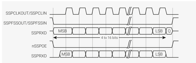
Figure 88. Motorola SPI frame format, single transfer, with SPO=0 and SPH=0
