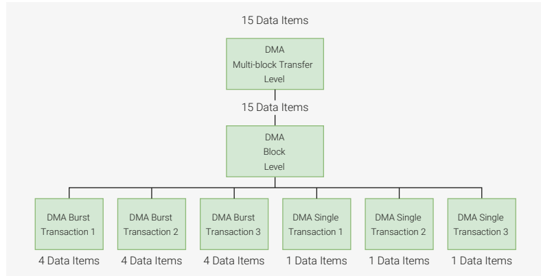
Figure 161. Breakdown of DMA Transfer into Single and Burst Transactions. Block size, DMA.CTLx.BLOCK_ TS = 15 . Number of data items per burst transaction, DMA.CTLx.DEST_M SIZE = 4 . SSI transmit FIFO watermark level, SSI.DMATDLR = DMA.CTLx.DEST_M SIZE = 4
