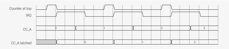
Figure 108. Each counter wrap causes the interrupt request signal to assert. The processor enters its interrupt handler, writes to its copy of the CC register, and clears the interrupt. When the counter wraps again, the latched version of the CC register is instantaneously updated with the most recent value written by software, and this value controls the duty cycle for the next period. The IRQ is reasserted so that software can write another fresh value to its copy of the CC register.
