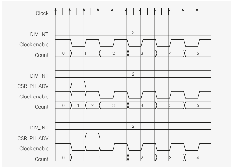
Figure 111. The clock enable signal, output by the clock divider, controls the rate of counting. Phase advance forces the clock enable high on cycles where it is low, causing the counter to jump forward by one count. Phase retard forces the clock enable low when it would be high, holding the counter back by one count.
