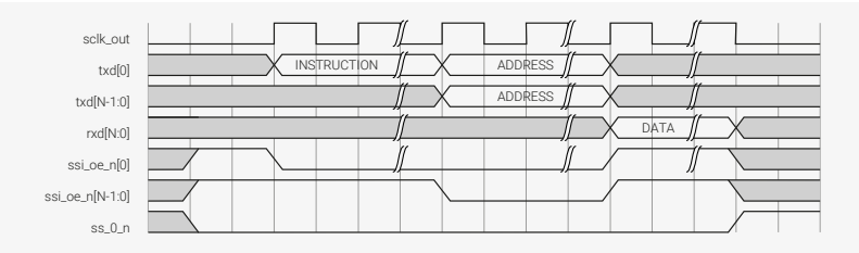
Figure 150. Instruction Transmitted in Standard and Address Transmitted in Enhanced SPI Format
