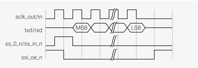
Figure 128. SSP Serial Format
